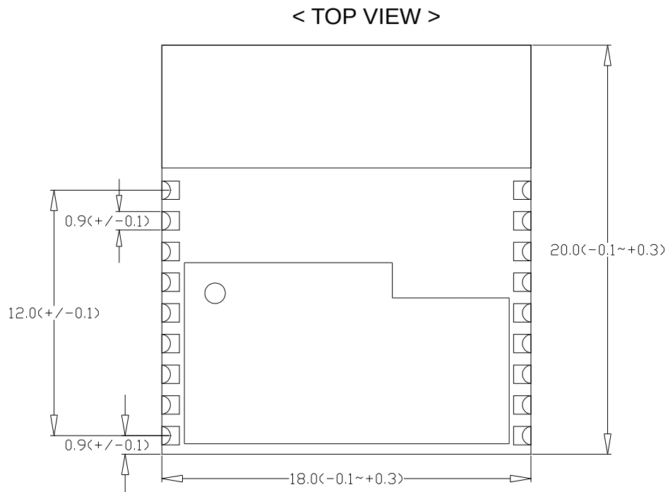
Figure 5-1 Physical Dimensions
