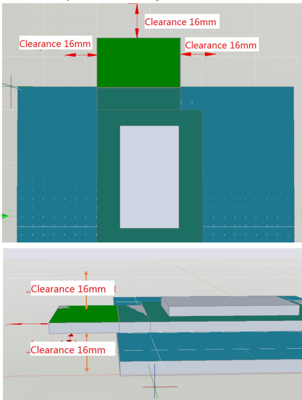
Figure 6-2 Antenna clearance reference
