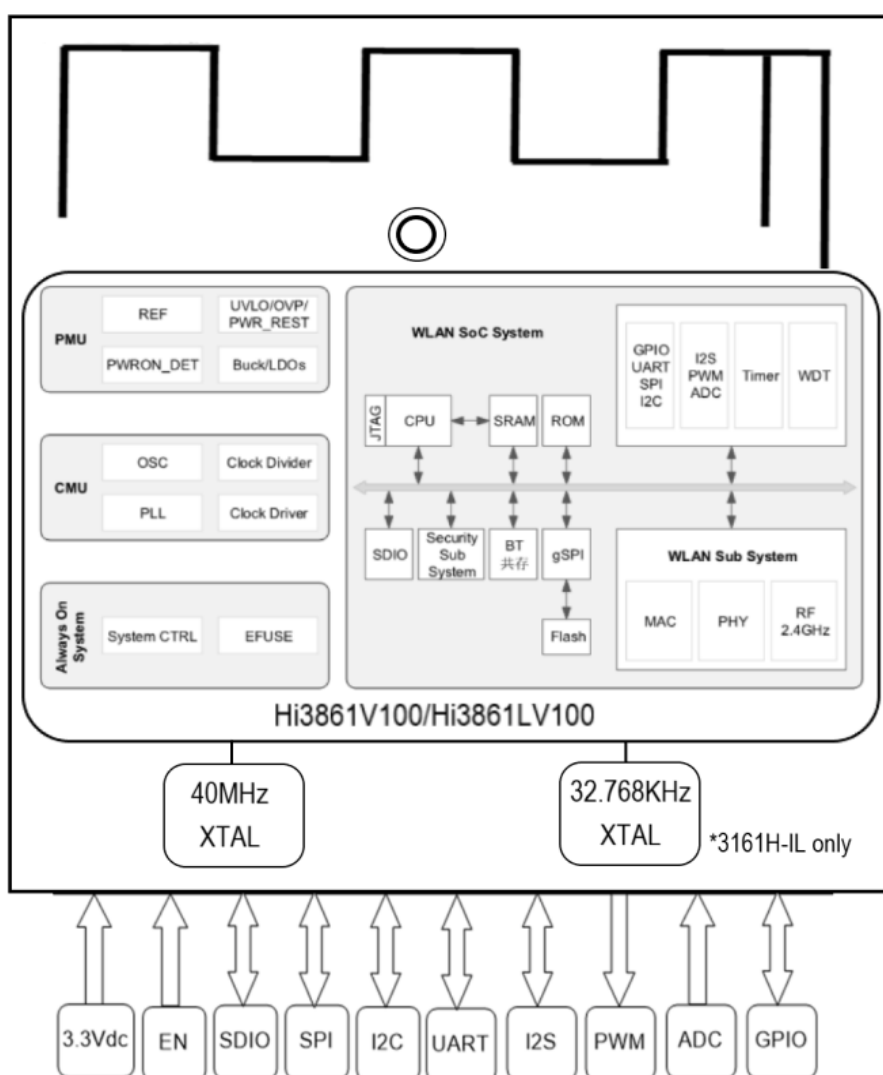
Figure 1-1 Block Diagram
