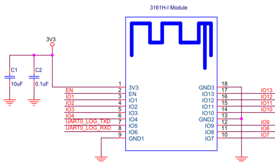
Figure 6-1 Reference Schematic
